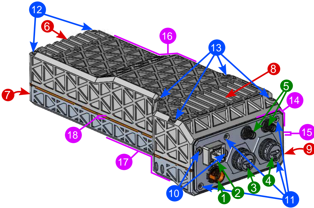
Figure 1. Components of an EDGETAK rev01
