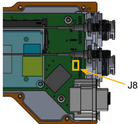
Figure 8. Jumper J8 on EDGETAK board
