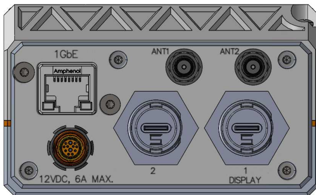
Figure 7. EDGETAK faceplate showing USB C connectors 1 and 2
