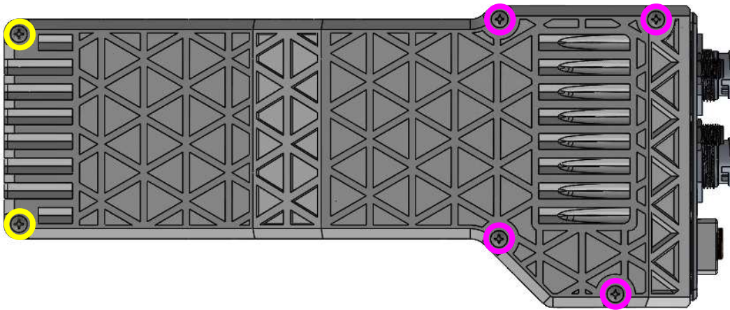
Figure 13. EDGETAK top clamshell enclosure screws
