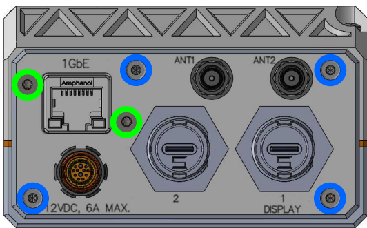
Figure 14. EDGETAK face plate screws
